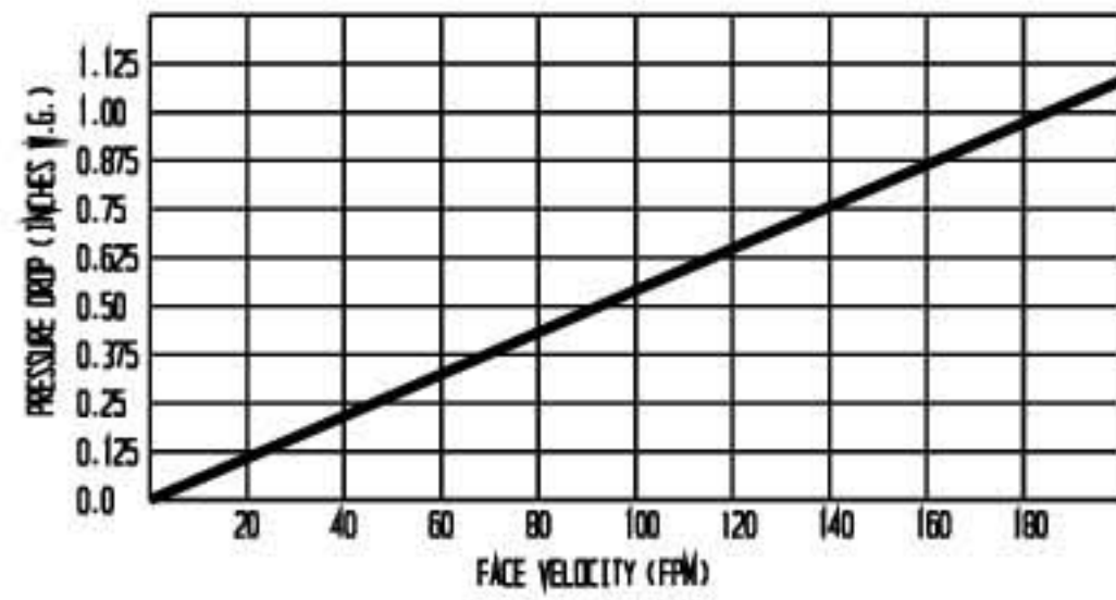
PRESSURE DROP VS. FACE VELOCITY HEPA FILTER 2" THK., 99.99% @ 0.3 MICRONS
