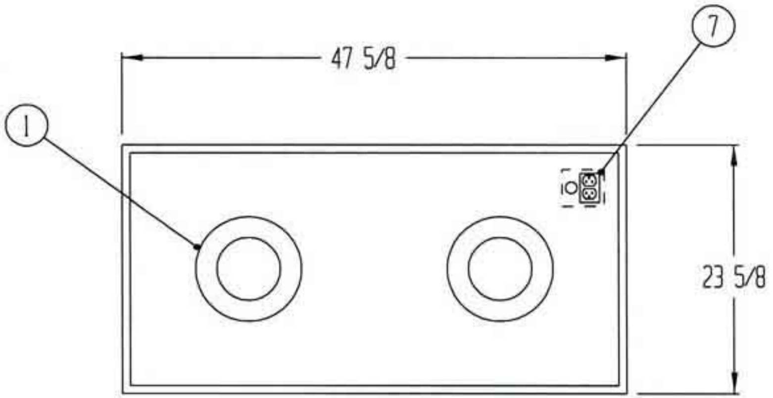
PLAN VIEW
