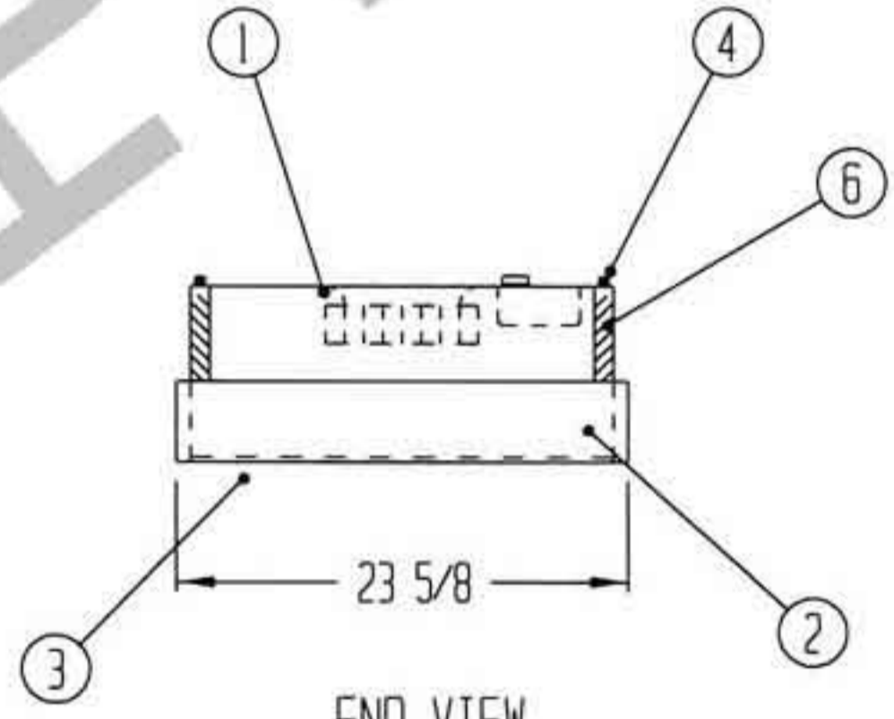
END VIEW
